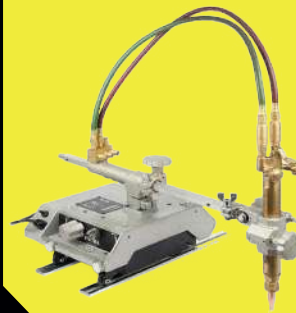
Straight gas cutting machine
